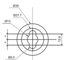
MOUNTING HOLE DETAILS SUITABLE FOR M12 BOLT
