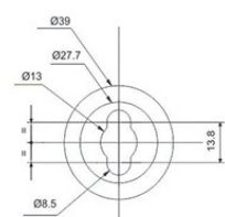
MOUNTING HOLE DETAILS SUITABLE FOR M12 BOLT
